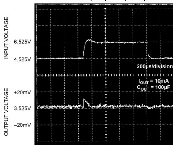
MIC29712 Line Transient Response with 100mA Load, 100μF Output Capacitance
