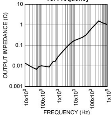
MIC29710/2 Output Impedance vs. Frequency
