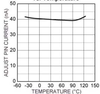
MIC29712 Adjust Pin Current vs. Temperature
