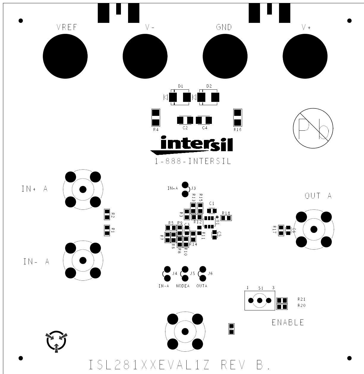
FIGURE 5. TOP VIEW
