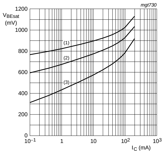
Fig 2. BCV63B: Base-emitter voltage as a function of collector current; typical values
