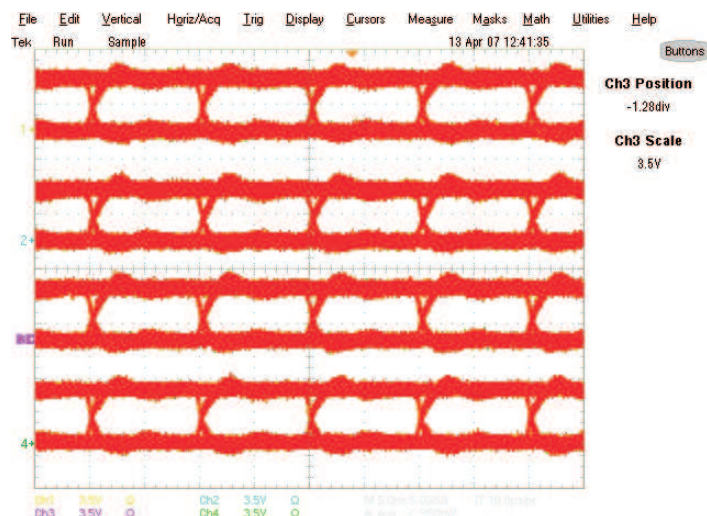
Figure 12. Typical Eye Patterns SN65LVDS3486: ( T = 25^{\circ}\text{C} ; V_{\text{CC}} = 3.6\text{ V} ; PRBS = 2^{23-1} )
