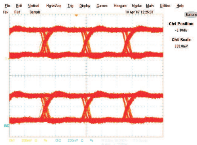
Figure 13. Typical Eye Patterns SN65LVDS9637: ( T = 25^{\circ}\text{C} ; V_{\text{CC}} = 3.6\text{ V} ; PRBS = 2^{23-1} )
