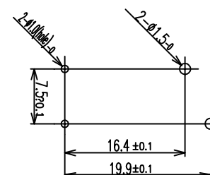
DRILLING DIAGRAM BOTTOM VIEW (2/1)
