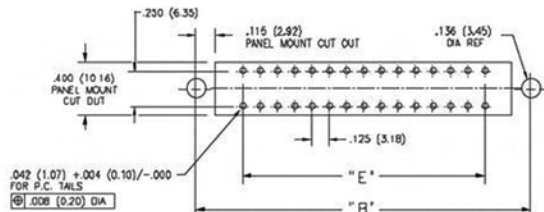
CONNECTOR MOUNTING PATTERN
