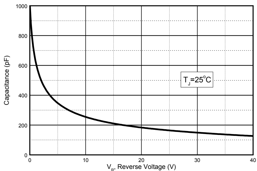
Figure 6. Capacitance
