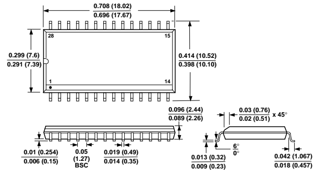
28-Pin Plastic SOIC (R-28)
