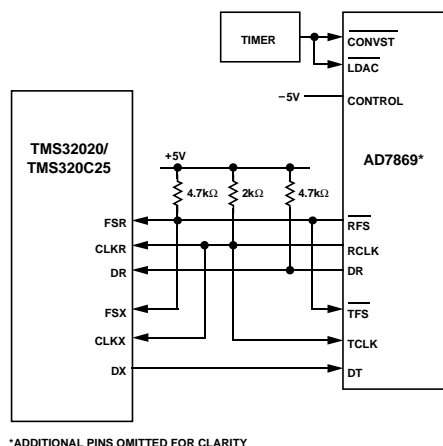
Figure 18. AD7869-TMS32020/TMS320C25 Interface
