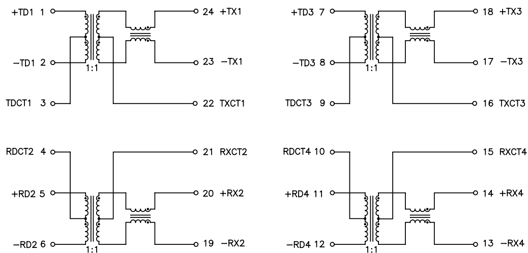
SCHEMATIC
