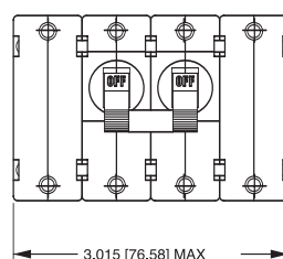
4-POLE (AB4)
