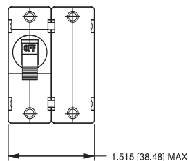
2-POLE (AB2)
