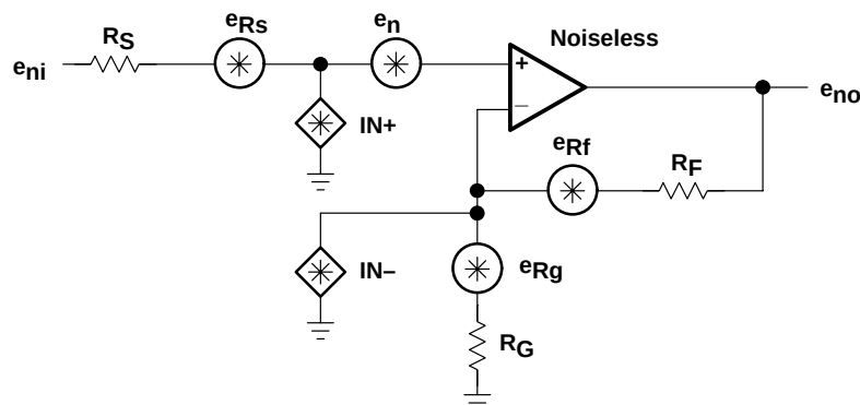
Figure 39. Noise Model
