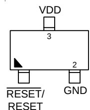
SOT-23-3 (L-Type)
