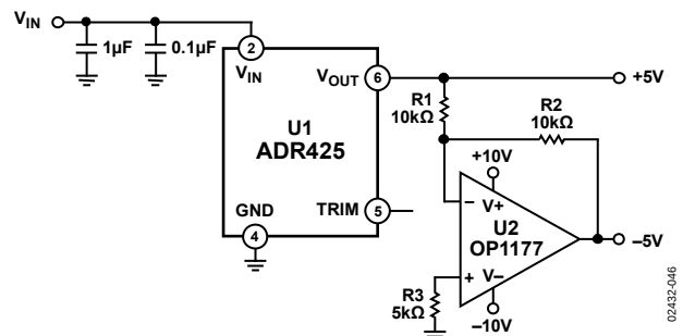
Figure 45. +5 V and -5 V Reference Using ADR425
