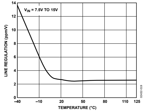
Figure 18. ADR425 Line Regulation vs. Temperature
