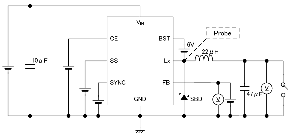
Circuit⑤
