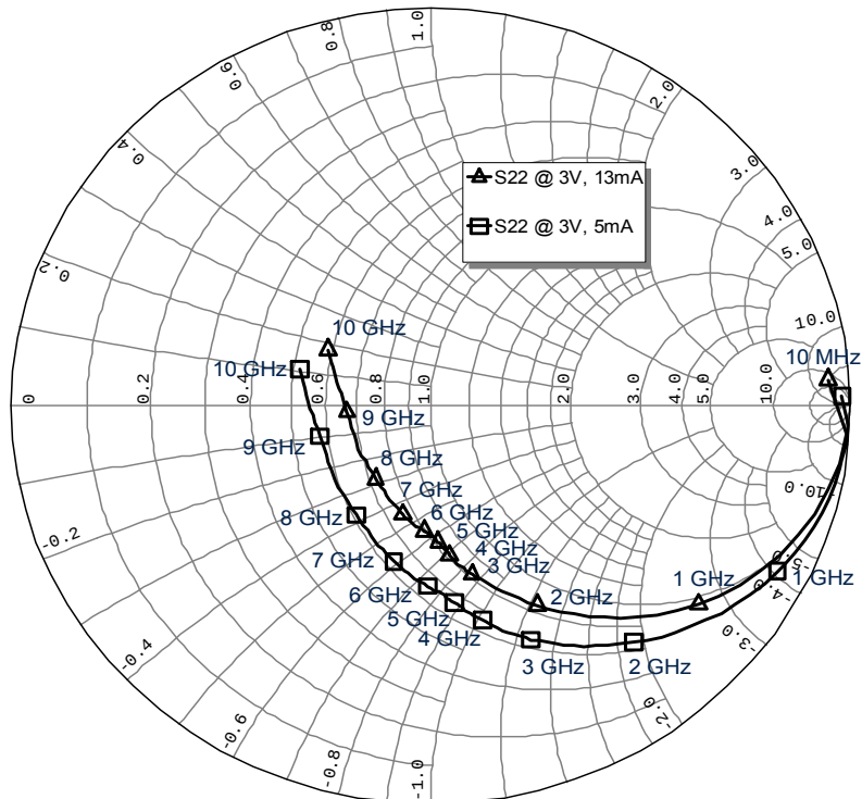
Figure 5-7 Output Matching S_{22} = f(f) , V_{CE} = 3\text{ V} , I_C = 5\text{ mA} / 13\text{ mA}
