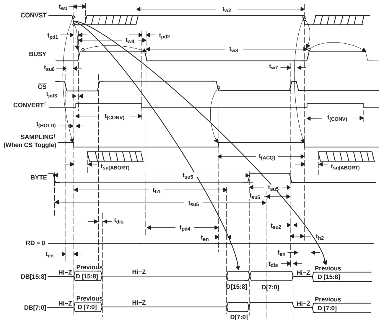
Figure 33. Timing for Conversion and Acquisition Cycles With \overline{\text{CS}} Toggling, \overline{\text{RD}} Tied to \text{BDGND}
