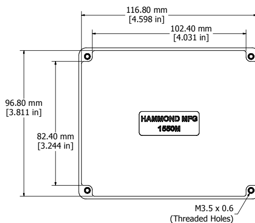
Top View Looking Inside Box
