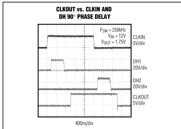
Figure 16. CLKOUT vs. CLKIN and DH 90° Phase Delay
