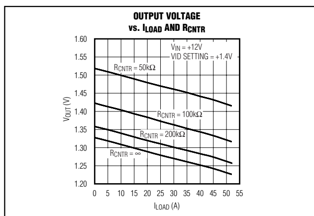
Figure 5. Output Voltage vs. I LOAD and RCNTR
