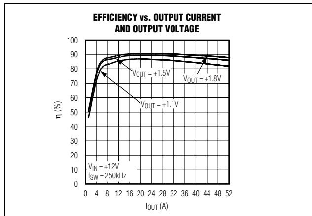
Figure 10. Efficiency vs. Output Current and Output Voltage
