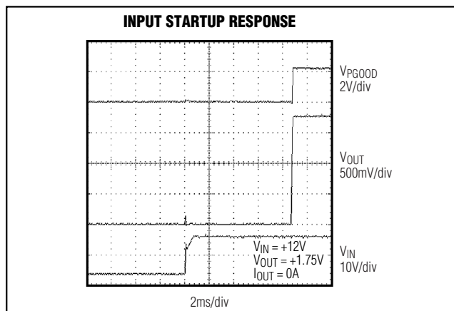
Figure 12. Input Startup Response
