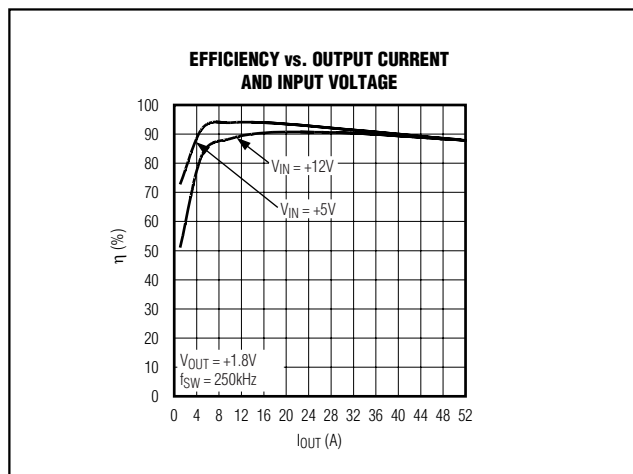
Figure 9. Efficiency vs. Output Current and Input Voltage
