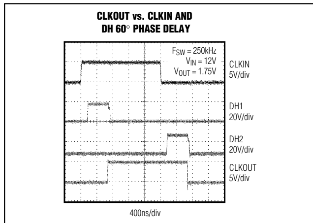
Figure 15. CLKOUT vs. CLKIN and DH 60° Phase Delay
