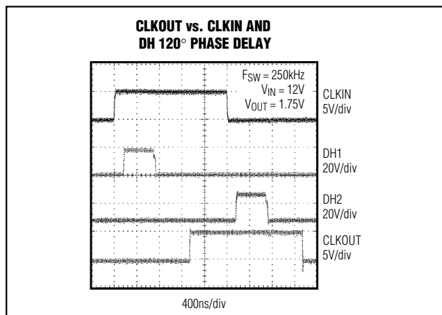
Figure 17. CLKOUT vs. CLKIN and DH 120° Phase Delay
