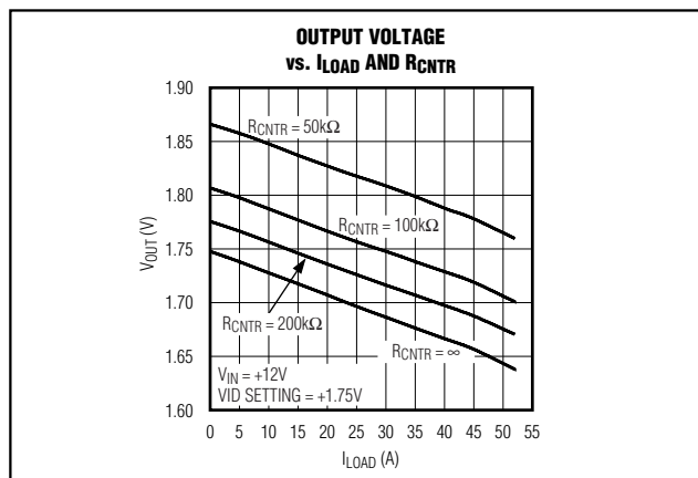
Figure 4. Output Voltage vs. I LOAD and RCNTR
