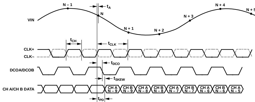
Figure 3. CMOS Interleaved Output Timing
