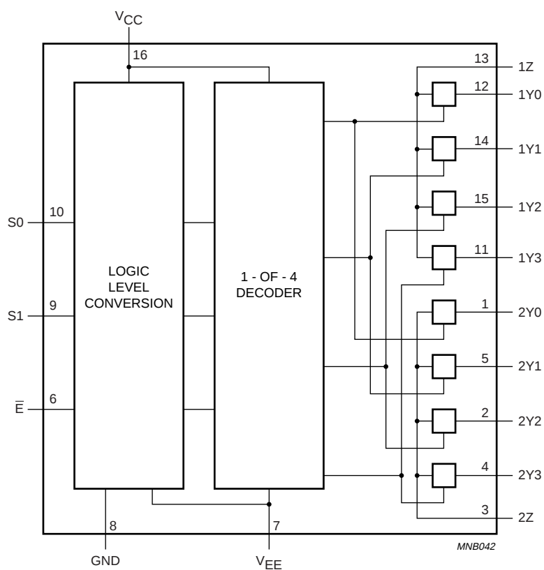
Fig.5 Functional diagram.
