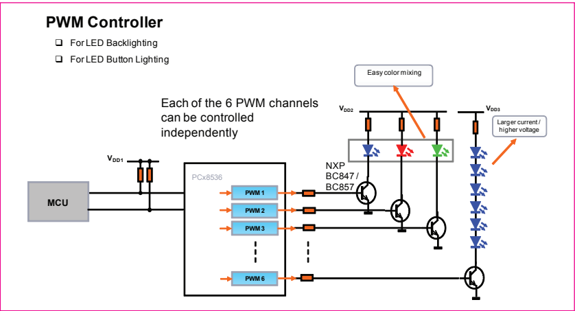
Integrated PWM controller for LED backlighting and button lighting
