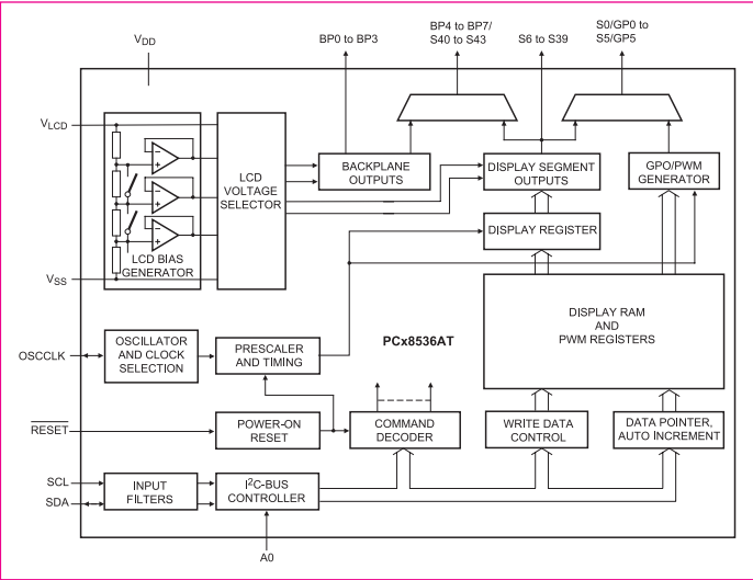
Integrated PWM controller for LED backlighting and button lighting
