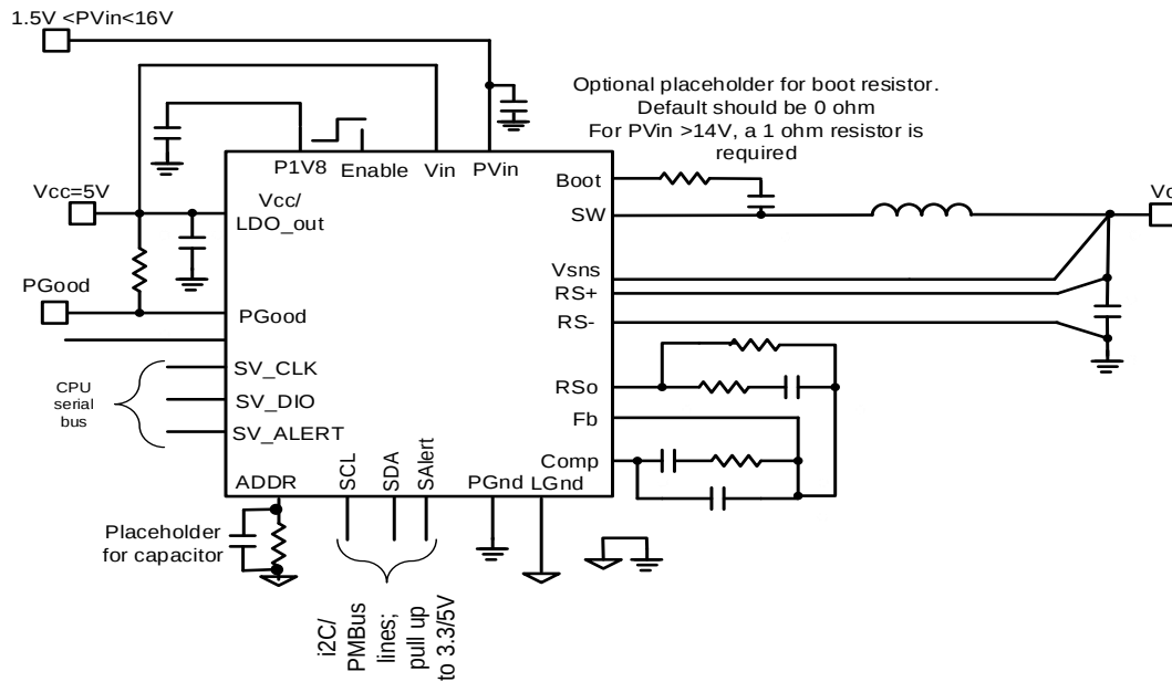
Figure 6: Using external Vcc, Vo<2.555V
