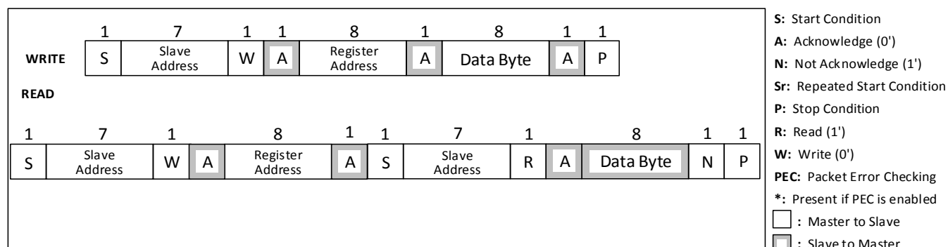
Figure 24: I2C Format
