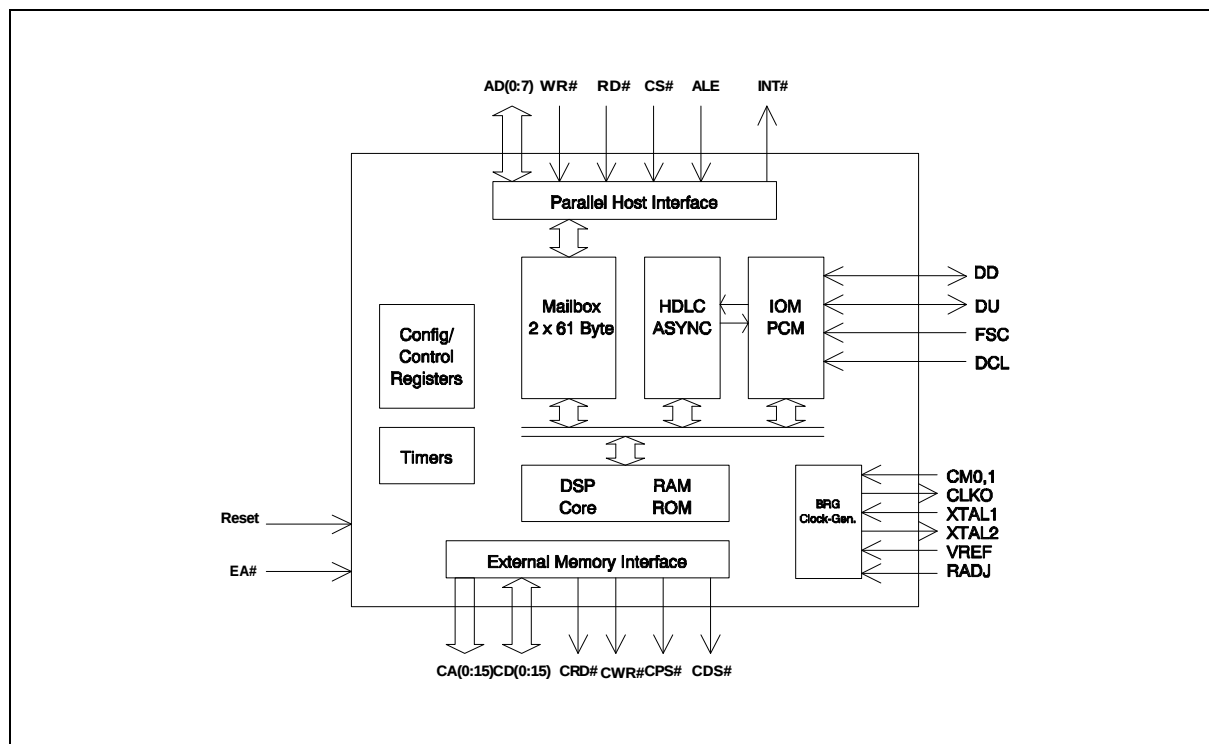
Figure 7 Device Architecture
