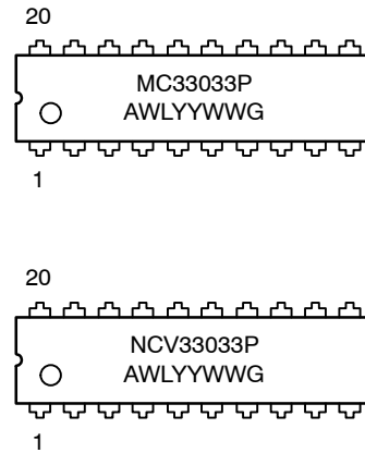
PDIP-20 P SUFFIX CASE 738
