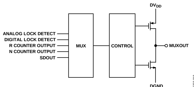
Figure 18. MUXOUT Circuit
