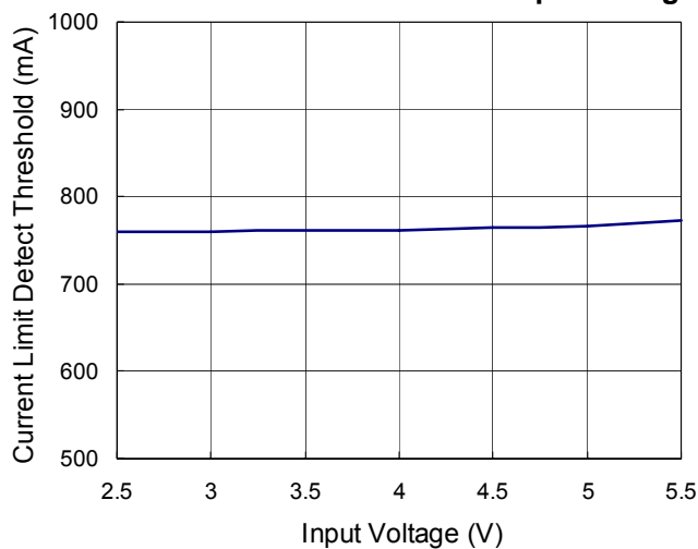
Current Limit Detect Threshold vs. Input Voltage
