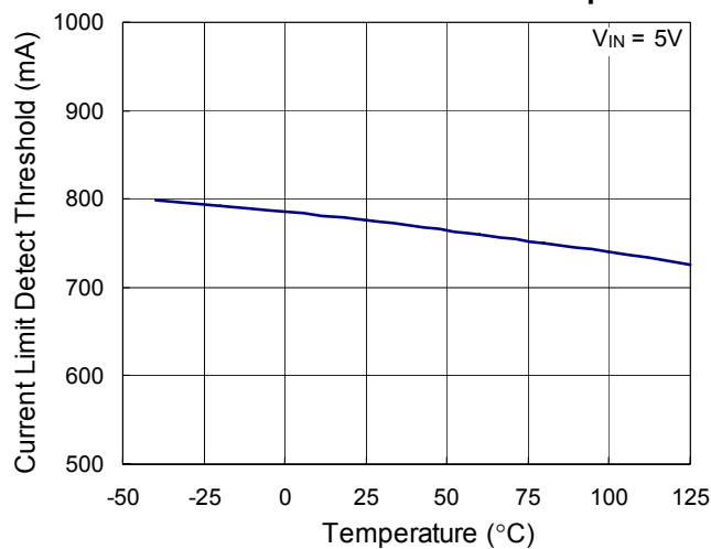
Current Limit Detect Threshold vs. Temperature
