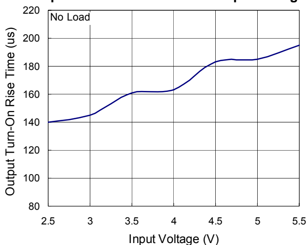
Output Turn-On Rise Time vs. Input Voltage
