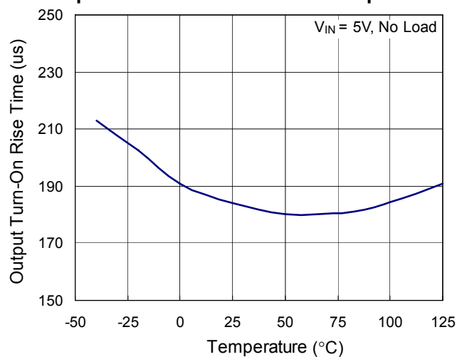
Output Turn-On Rise Time vs. Temperature
