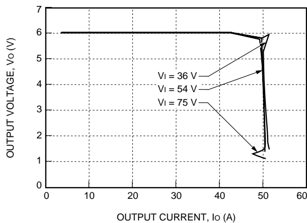
Figure 2. Typical FW250S6R0 Output Characteristics at Room Temperature
