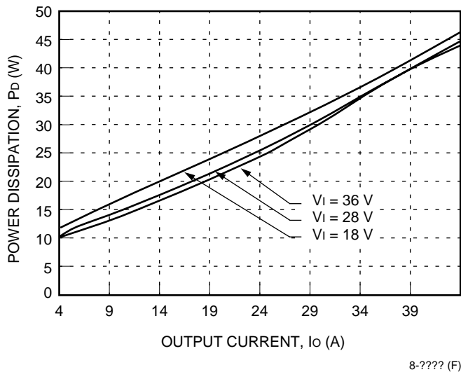
Figure 24. FW300S6R0 Power Dissipation vs. Output Current at 25 °C
