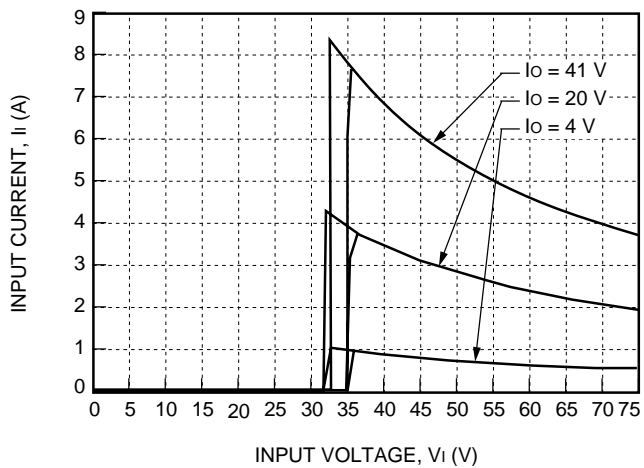
Figure 1. Typical FW250S6R0 Input Characteristics at Room Temperature
