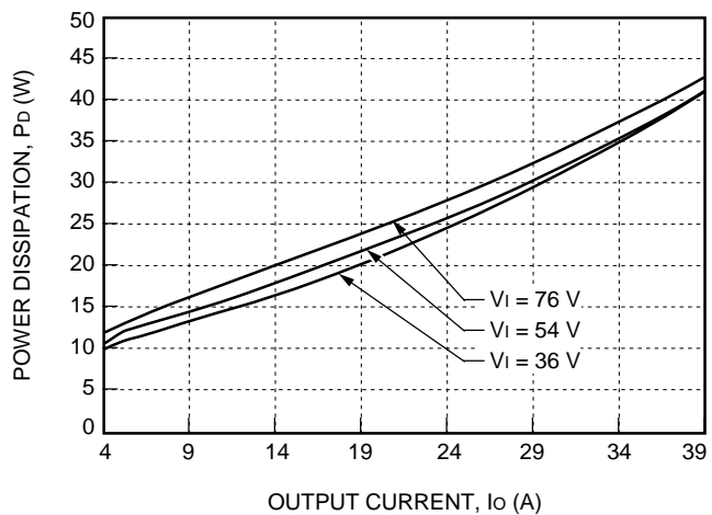
Figure 23. FW250S6R0 Power Dissipation vs. Output Current at 25 °C
