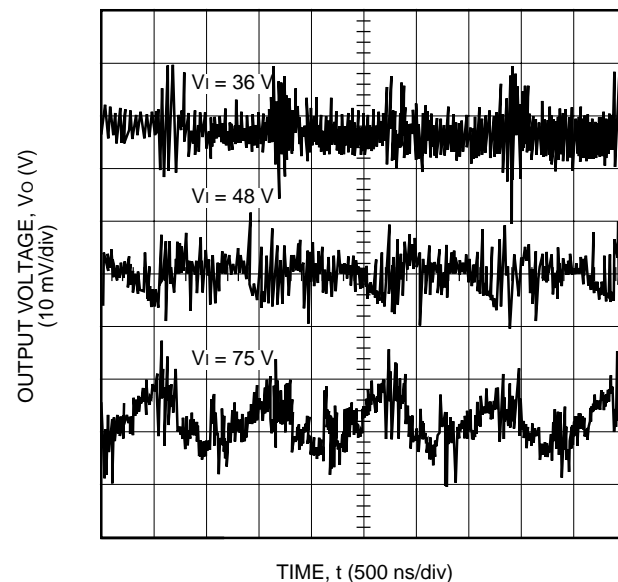
Figure 4. Typical FW250S6R0 Output Ripple Voltage at Room Temperature and 50 A Output
