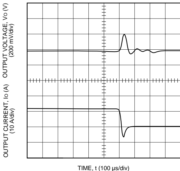
Figure 5. Typical FW250S6R0 Transient Response to Step Decrease in Load from 50% to 25% of Full Load at Room Temperature and 48 V Input (Waveform Averaged to Eliminate Ripple Component.)
