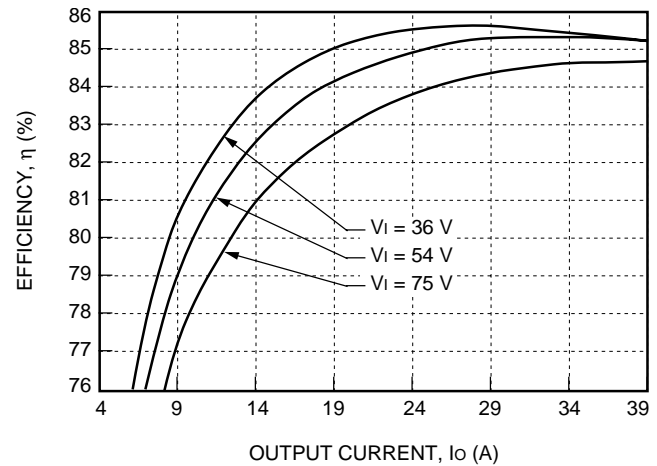
Figure 3. Typical FW250S6R0 Efficiency vs. Output Current at Room Temperature
