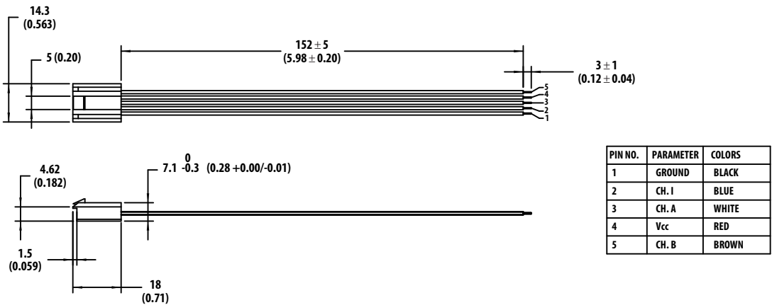
Figure 4. HEDS-8902 and HEDS-8903 Connectors
