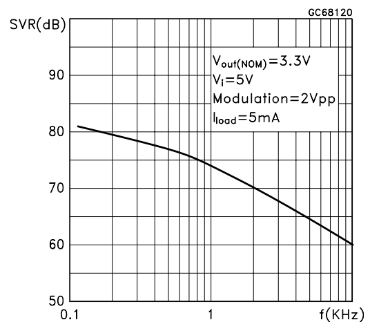
Figure 6 : S.V.R. vs Frequency
