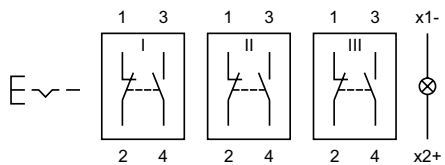
Wiring diagram 26
