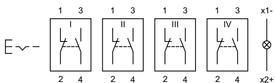
Wiring diagram 28
