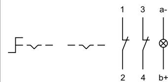
Wiring diagram 18
