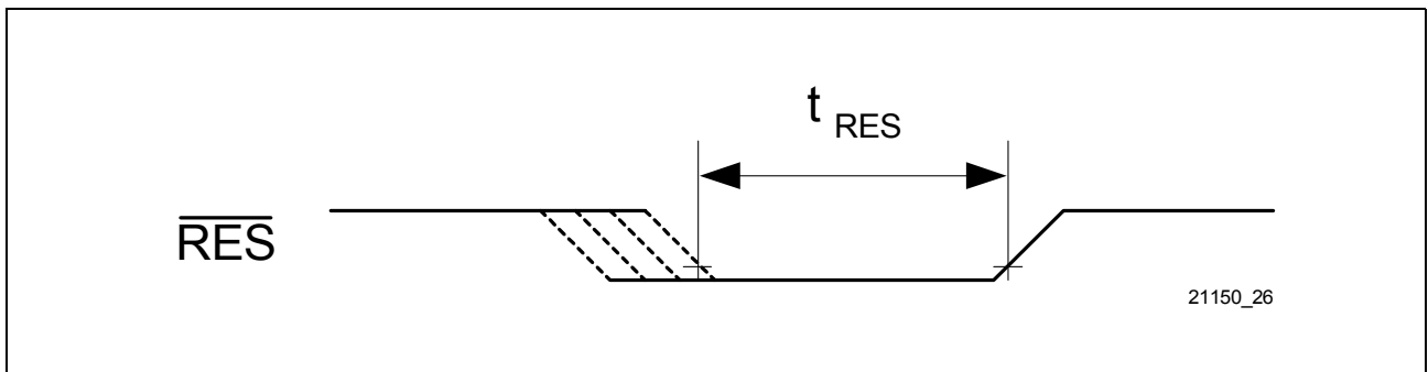
Figure 82 Reset Signal \overline{\text{RES}}
