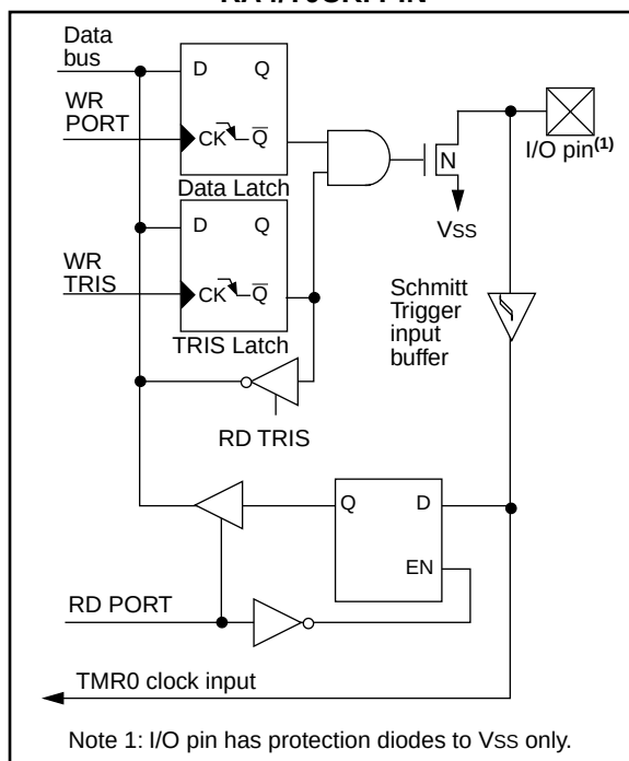
FIGURE 5-2: BLOCK DIAGRAM OF THE RA4/T0CKI PIN
