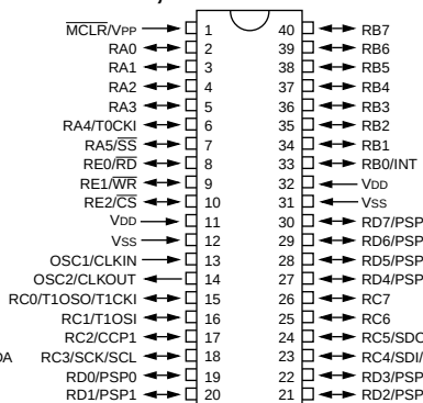
PIC16C64A PIC16CR64
