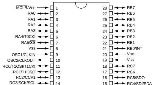
PIC16C62
