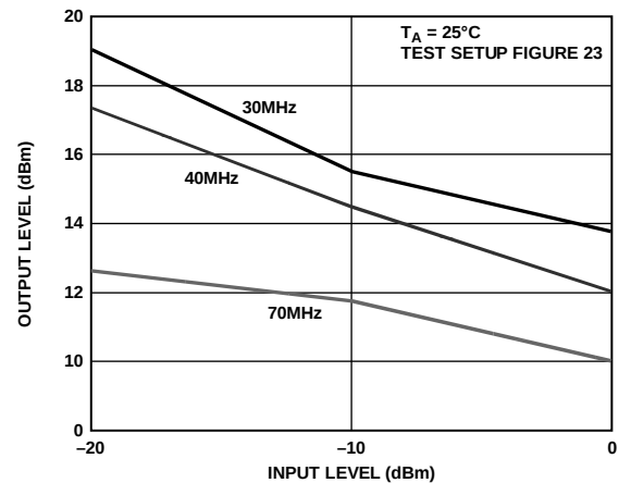
Figure 27. Third-Order Intercept -10 dB/+30 dB Mode, Gain = 10 dB
