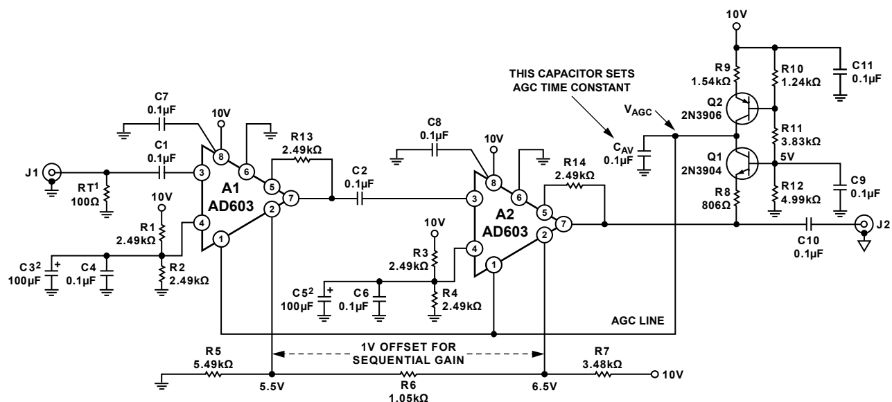
Figure 49. A Low Noise AGC Amplifier
