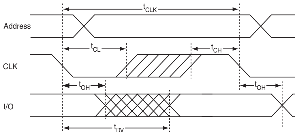
Figure 18-2. Read
