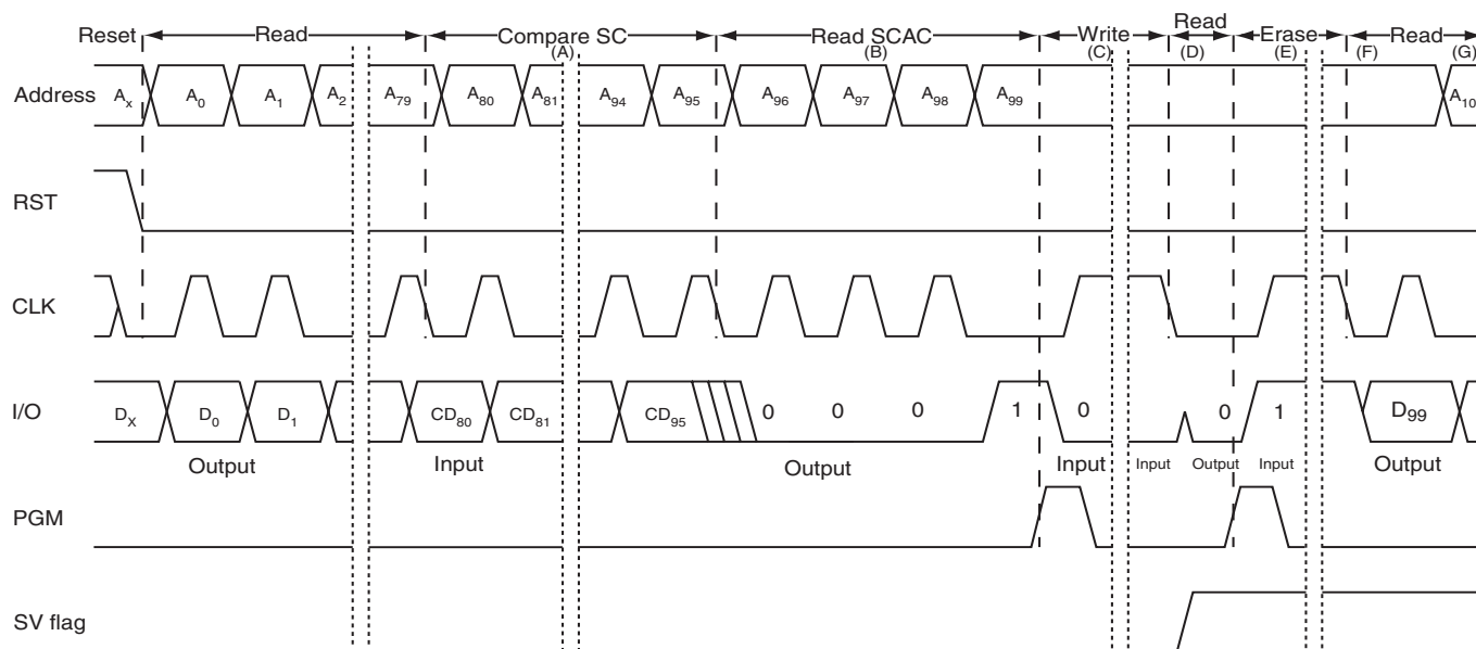
Figure 18-5. Security Code Validation
