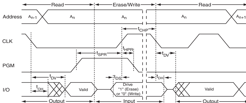
Figure 18-3. Erase/Write
