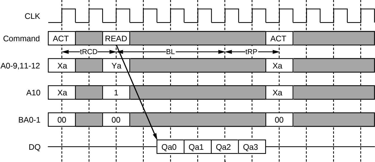
Read with Auto-Precharge (CL=2, BL=4)
