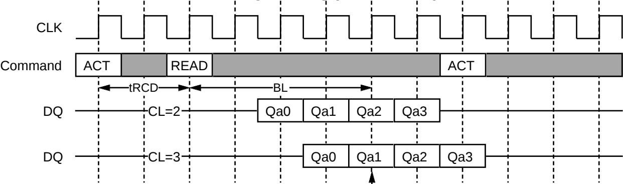
Auto-Precharge Timing (READ, BL=4)
