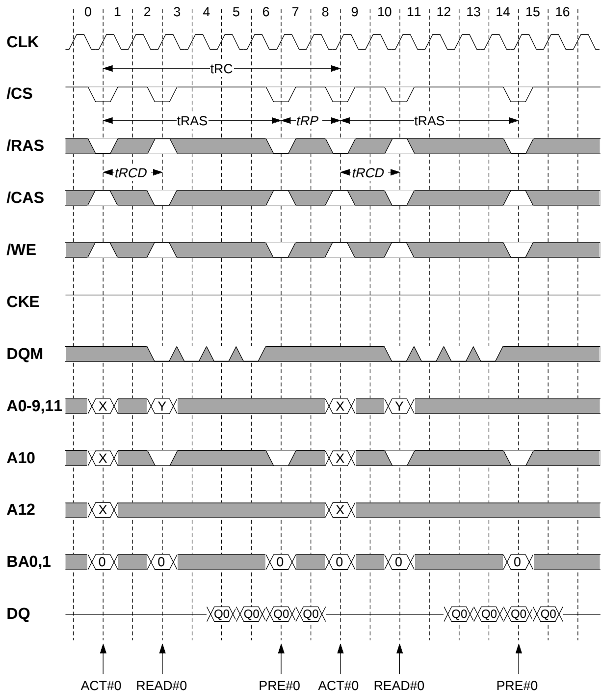
Burst Read (Single Bank) [CL=2, BL=4]
