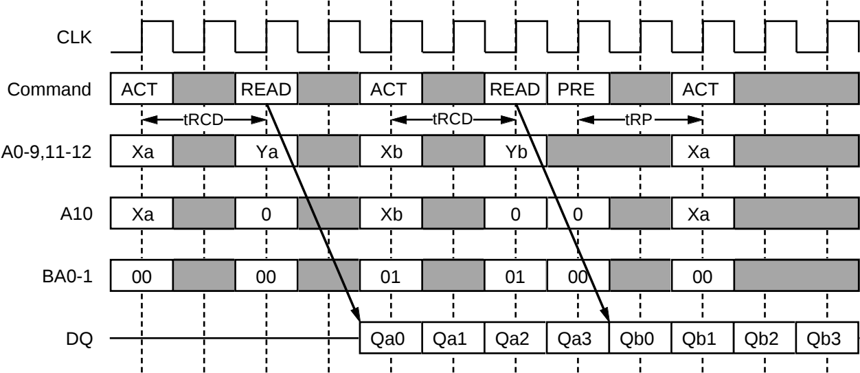
Multi Bank Interleaving Read (CL=2, BL=4)
