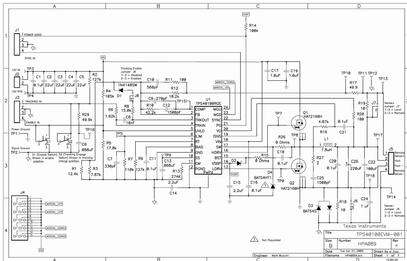
Figure 4-1. TPS40100EVM-001 Power Stage/Control Schematic
