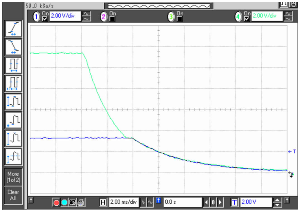
Figure 5-6. Single EVM Tracking Discharging Ramp
