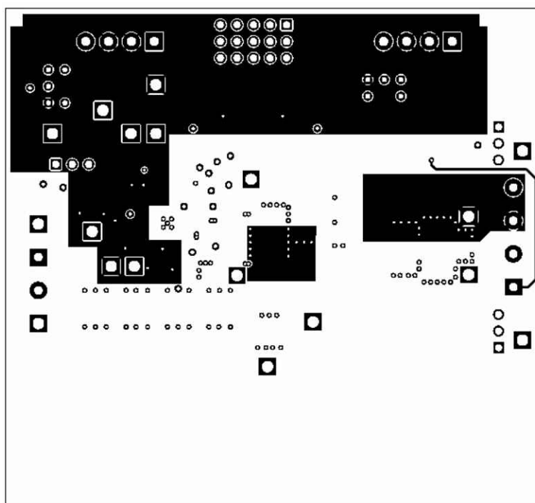
Figure 7-4. TPS40100EVM-001 Layer 2 (X-Ray View from Top)
