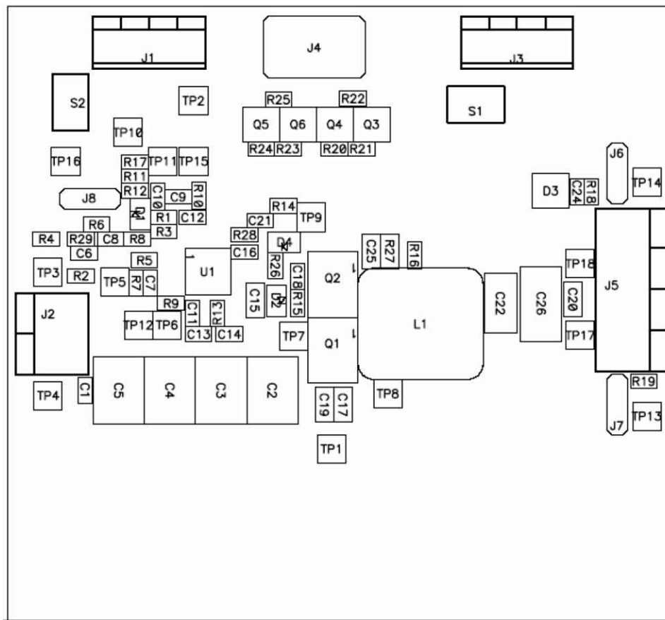
Figure 7-1. TPS40100EVM-001 Component Placement (Viewed from Top)
