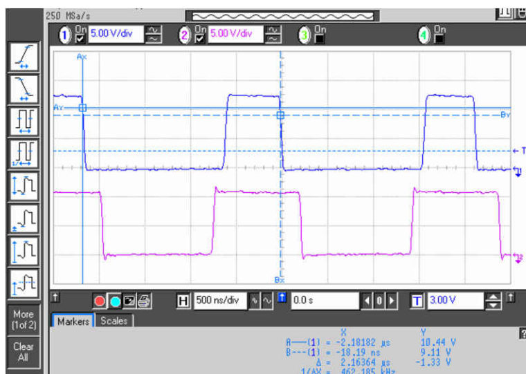
Figure 5-13. Synchronization
