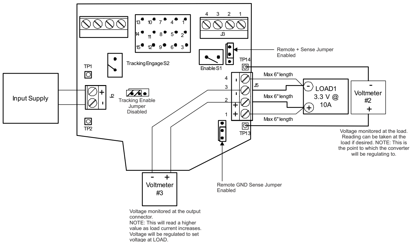
Figure 5-3. TPS40100EVM-001 Recommended Remote Test Setup
