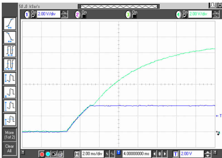
Figure 5-5. Single EVM Tracking Charging Ramp
