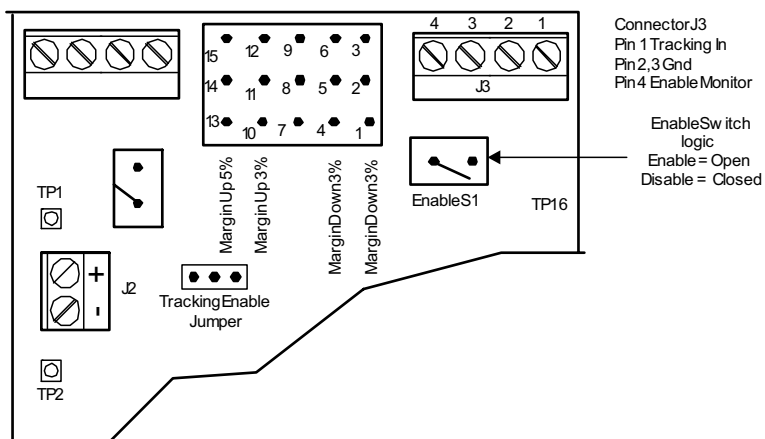
Figure 5-8. TPS40100EVM-001 Enable Test Setup
