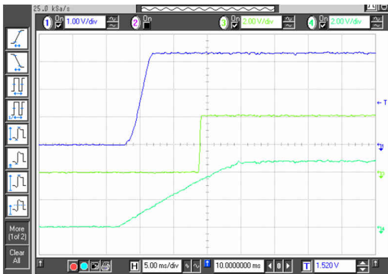
Figure 5-9. Power On from Enable
