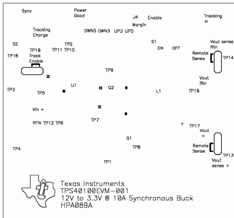
Figure 7-2. TPS40100EVM-001 Silkscreen (Viewed from Top)
