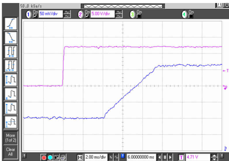
Figure 5-11. Margin Up 5%
