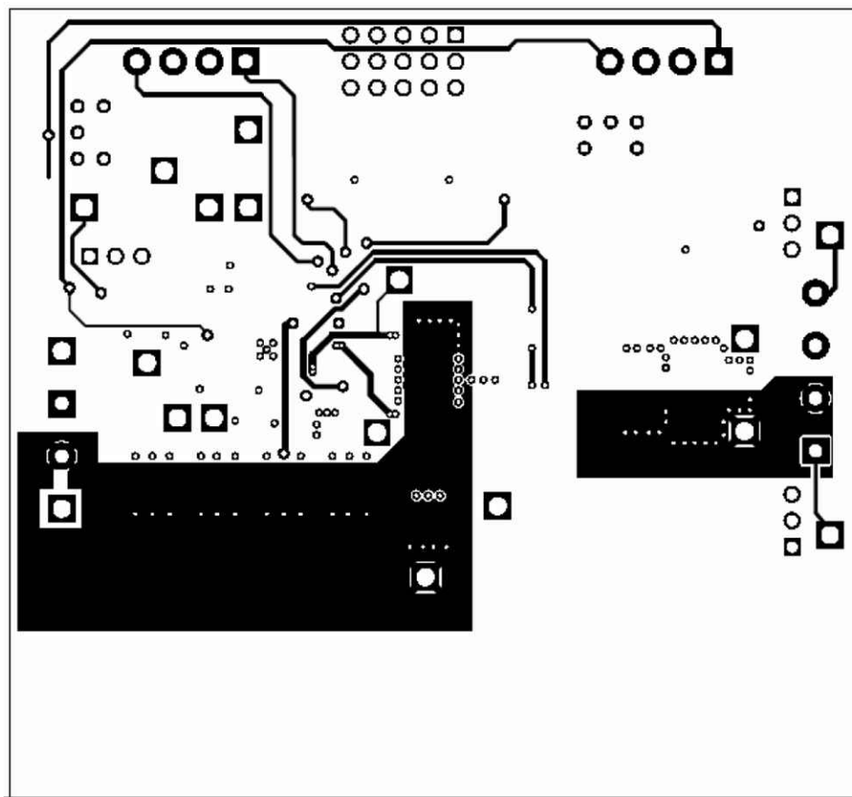
Figure 7-5. TPS40100EVM-001 Layer 3 (X-Ray View from Top)
