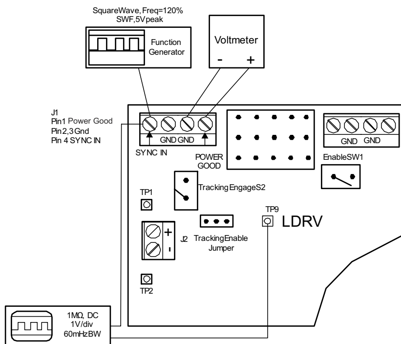
Figure 5-12. TPS40100EVM-001 Power Good and Synchronization Test Setup
