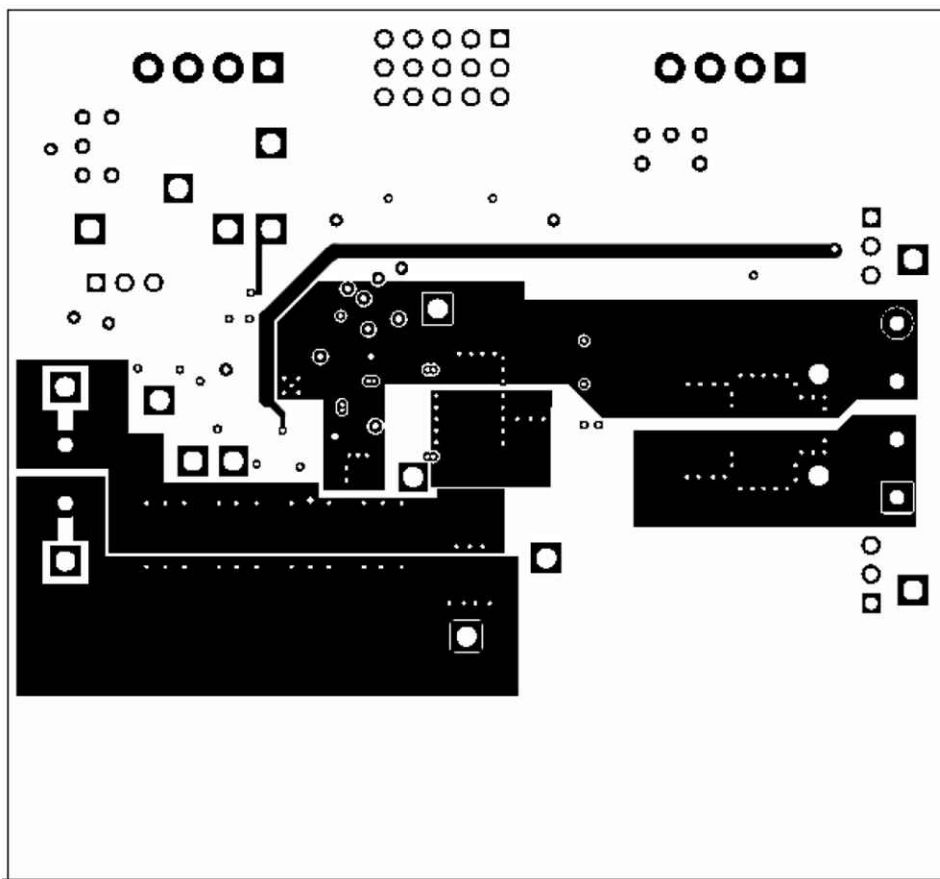
Figure 7-6. TPS40100EVM-001 Bottom Copper (X-Ray View from Top)
