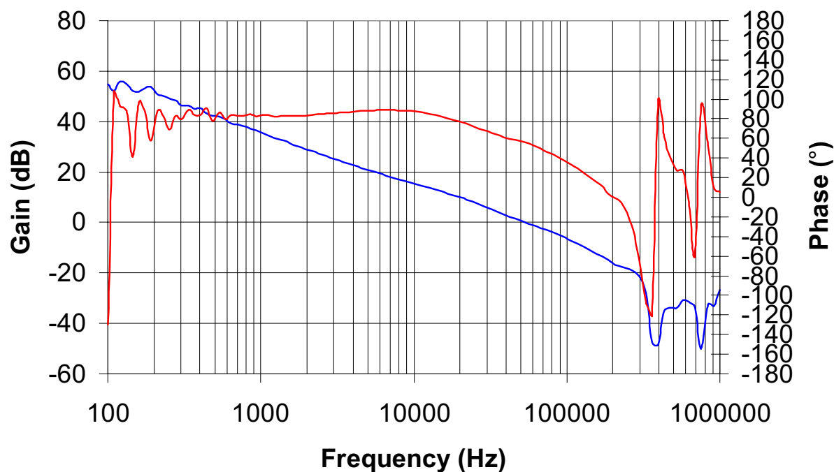
Figure 6-3. TPS40100EVM-001 Loop Response V_{IN} = 12\text{ V} , V_{OUT} = 3.3\text{ V} , I_{OUT} = 10\text{ A}
