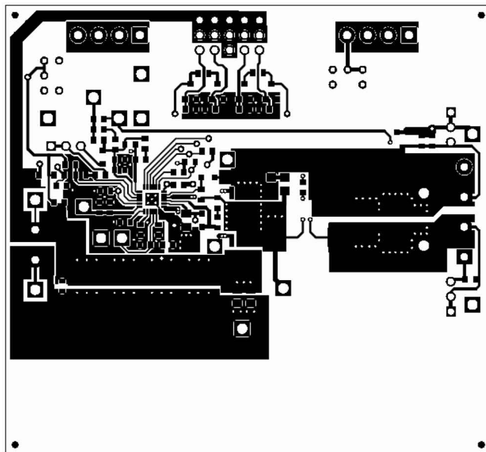
Figure 7-3. TPS40100EVM-001 Top Copper (Viewed from Top)
