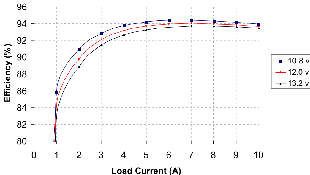
Figure 6-1. TPS40100EVM-001 Efficiency V_{12V\_IN} = 10.8\text{ V} - 13.2\text{ V} , V_{OUT} = 3.3\text{ V} , I_{OUT} = 0\text{ A} - 10\text{ A}
