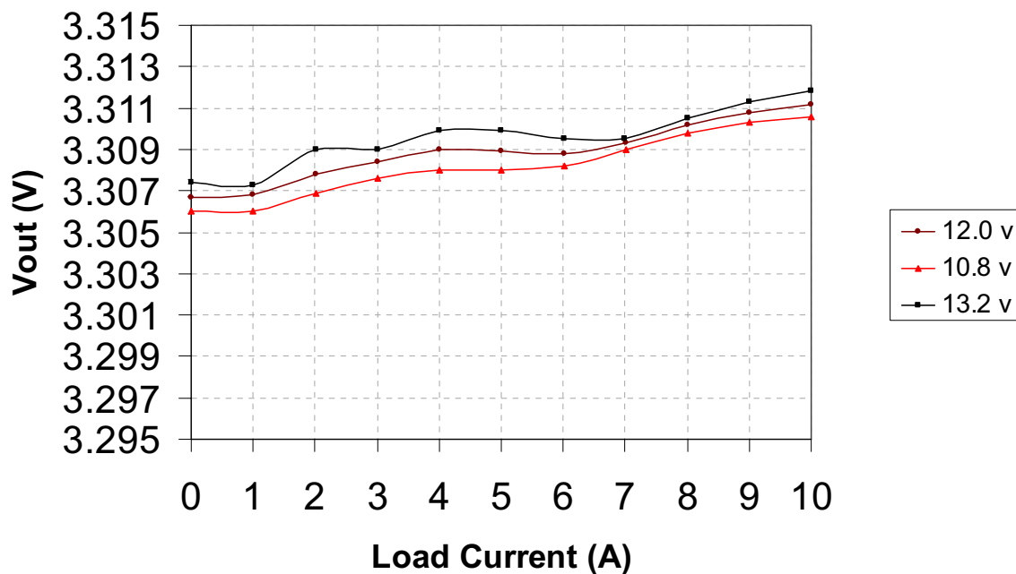
Figure 6-2. TPS40100EVM-001 Line Regulation I_{OUT} = 10\text{ A} , V_{IN} = 10.8\text{ V} - 13.2\text{ V}
