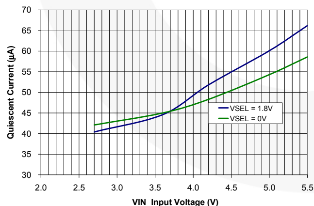
Figure 15. Quiescent Current, I_{LOAD} = 0 , EN = 1.8\text{ V}
