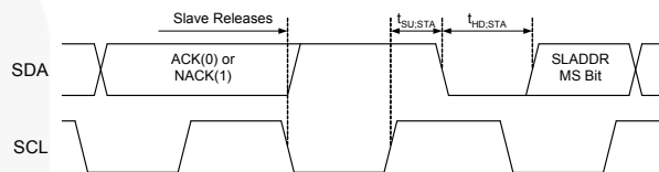
Figure 44. Repeated-Start Timing
