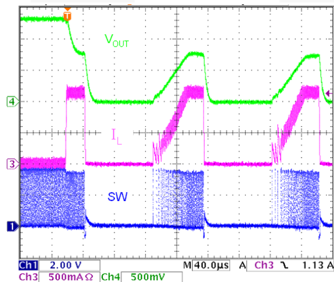
Figure 31. R_{LOAD} = 660 mΩ
