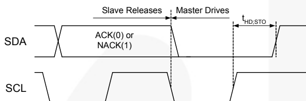
Figure 43. Stop Bit
