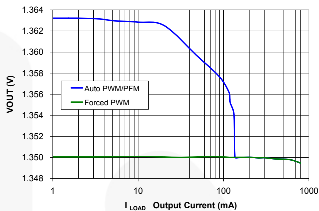
Figure 12. Load Regulation at V_{OUT} = 1.35\text{ V}
