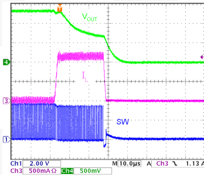
Figure 32. R_{LOAD} = 660 mΩ
