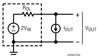
Figure 2. Equivalent Open-Loop Circuit
