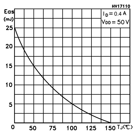
Figure 14. Maximum avalanche energy vs temperature
