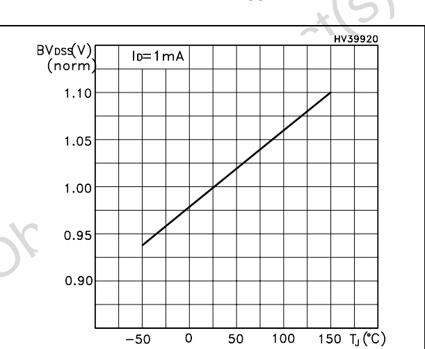
Figure 17. Normalized B_{VDS} vs temperature
