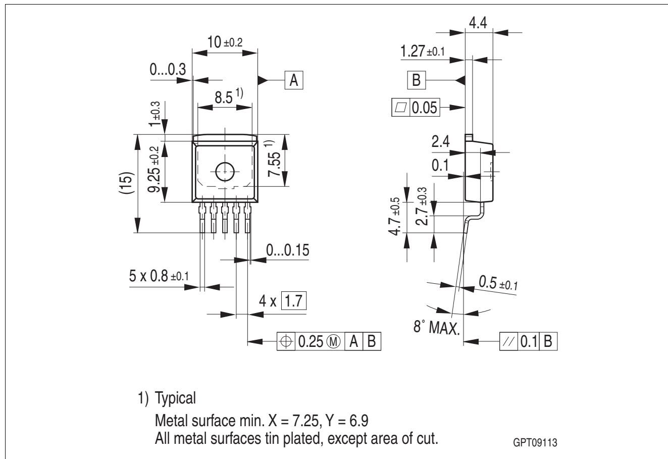
Figure 5 PG-TO263-5 SMD Package
