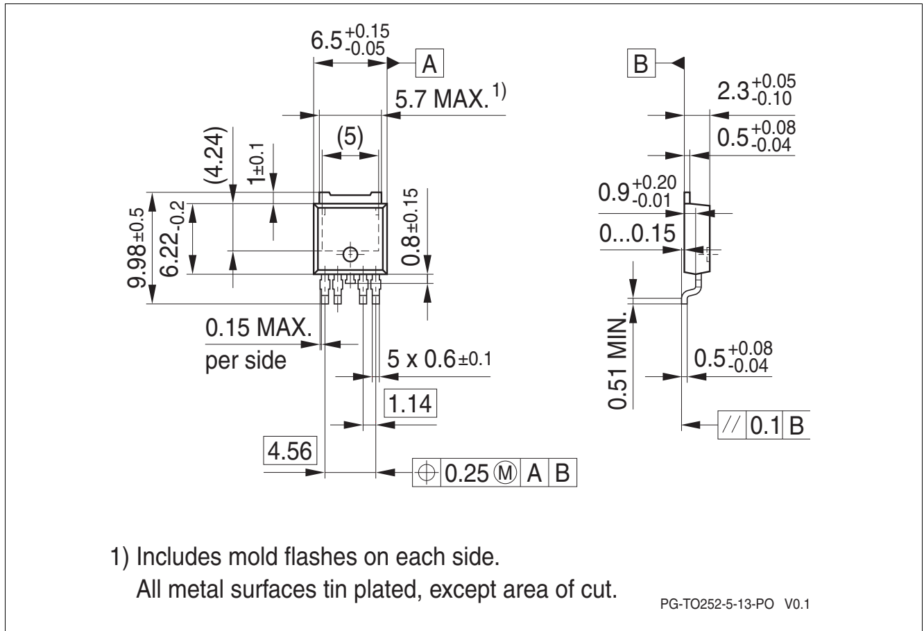
Figure 6 PG-TO252-5 SMD Package
