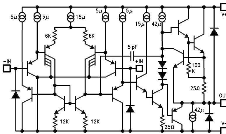
Figure 69. Op Amp
