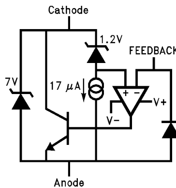
Figure 54. Reference Equivalent Circuit
