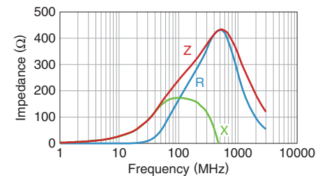
MMZ1005Y241C
