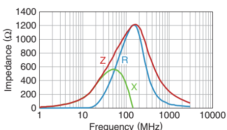
MMZ1608Y102B
