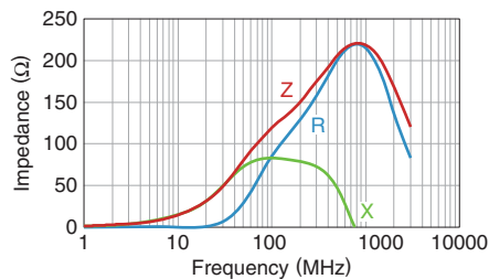
MMZ1005Y121C
