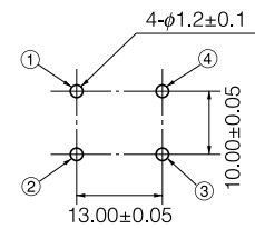
Recommended PWB piercing plan
