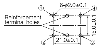
Recommended PWB piercing plan
