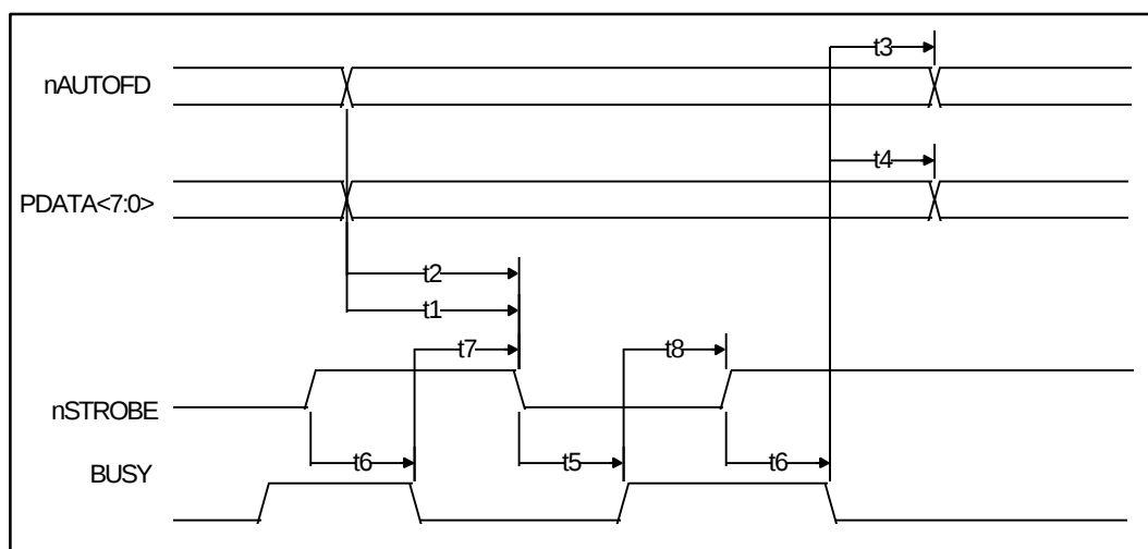
FIGURE 65 - ECP PARALLEL PORT FORWARD TIMING
