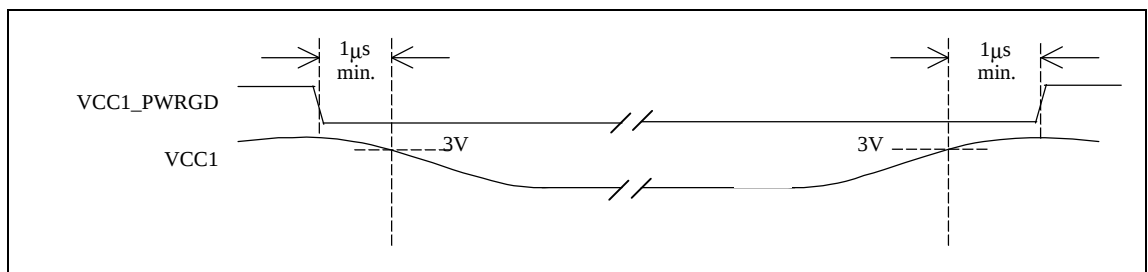
FIGURE 5 - VCC1_PWRGD TIMING
