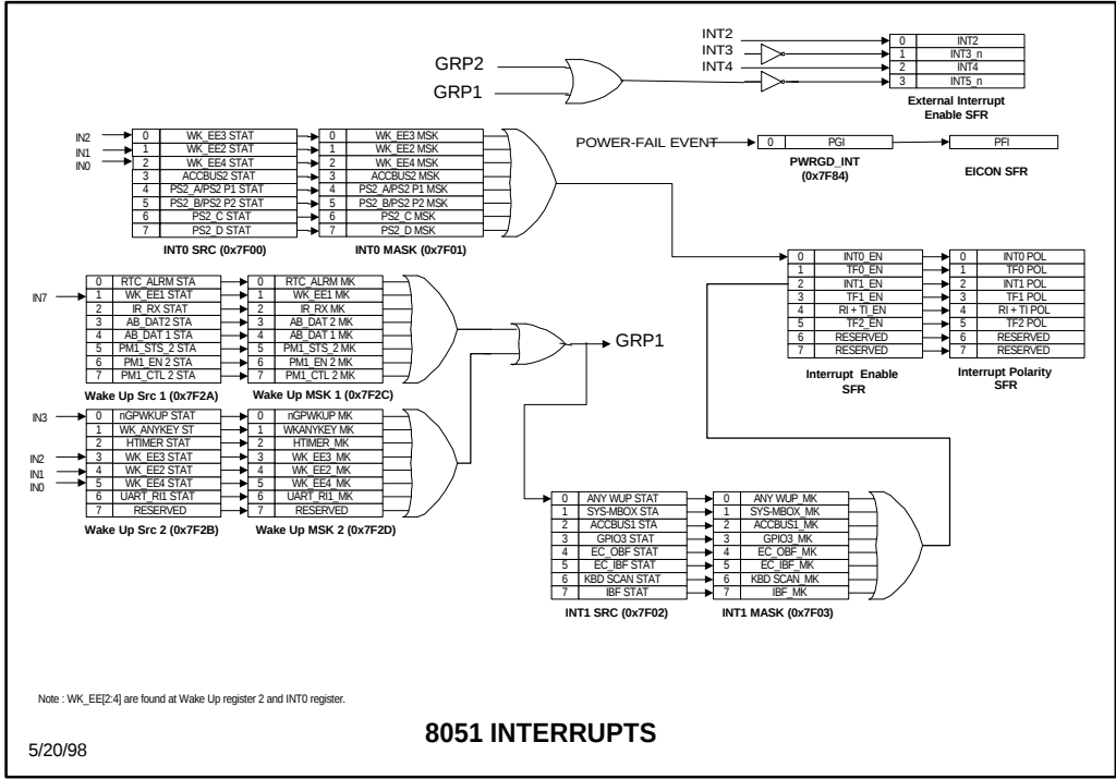
FIGURE 19 - 8051 INTERRUPTS
