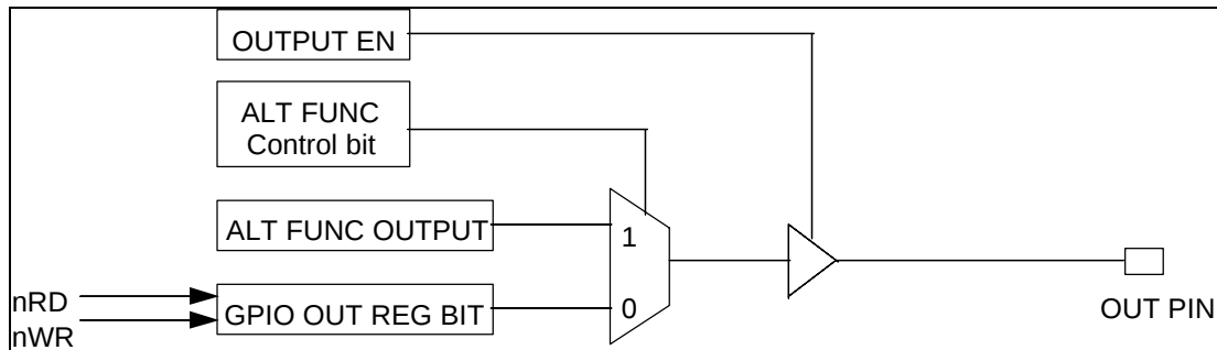
FIGURE 38 - OUTPUT PIN TYPE
