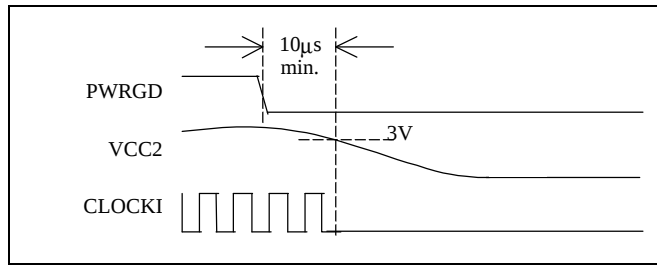
FIGURE 3 – POWER-FAIL EVENT
