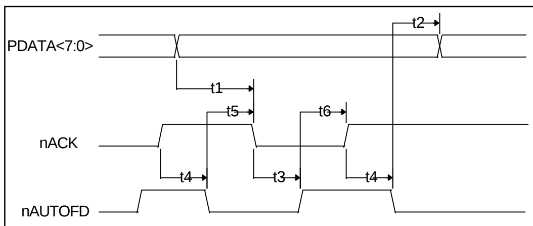
FIGURE 66 - ECP PARALLEL PORT REVERSE TIMING
