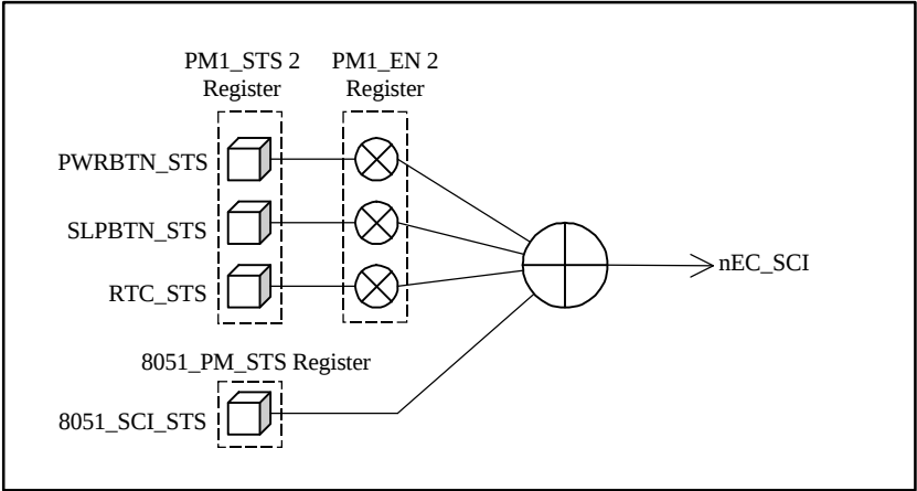
FIGURE 45 - HARDWARE nEC_SCI INTERFACE
