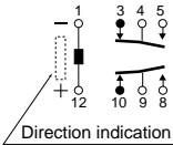
1 coil latching (Reset condition)
