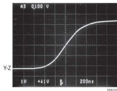
Figure 18. Driver Differential Output. R = 27\Omega , V_{CC2} = 5V , \overline{SLO} = 0V
