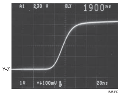
Figure 17. Driver Differential Output. R = 27\Omega , V_{CC2} = 5V , \overline{SLO} = V_{CC2}
