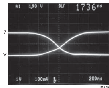
Figure 16. Driver Output. R = 27\Omega , V_{CC2} = 5V , \overline{SLO} = 0V
