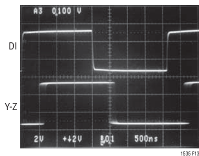
Figure 13. Driver Propagation Delay with Sample Jitter. \overline{SLO} = V_{CC2}
