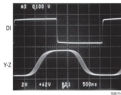
Figure 14. Driver Propagation Delay with Sample Jitter. \overline{SLO} = 0V
