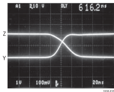
Figure 15. Driver Output. R = 27\Omega , V_{CC2} = 5V , \overline{SLO} = V_{CC2}
