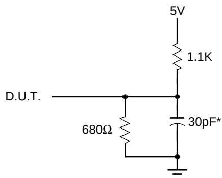
Figure 1. Output Load
