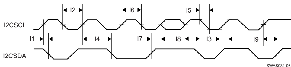
Figure 4-18. I 2 C Timing
