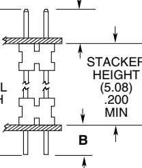
POST HEIGHT (1.65) .065 MIN
